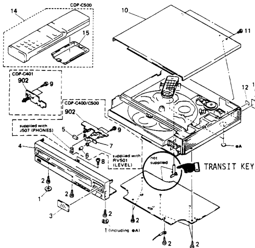
5-1. FRONT PANEL ASSEMBLY AND COVERS
